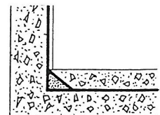
FOUNDATIONS, SPLIT SLAB APPLICATIONS
