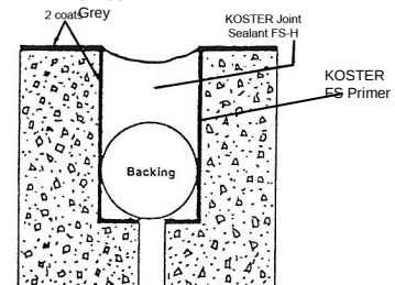
KOSTER NB 1 Grey - 2 coats. Allow KOSTER NB 1 Grey to cure a minimum period of 72 hours before applying backing and sealant.
